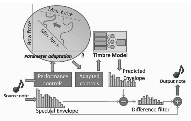
Figure 5: Schema for timbre transformation: a) shift and adapt controls, b) predict new timbre, and c) filter
