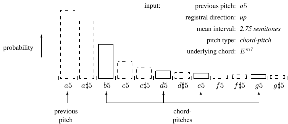
Figure 3: Probability distribution for pitch-selection
