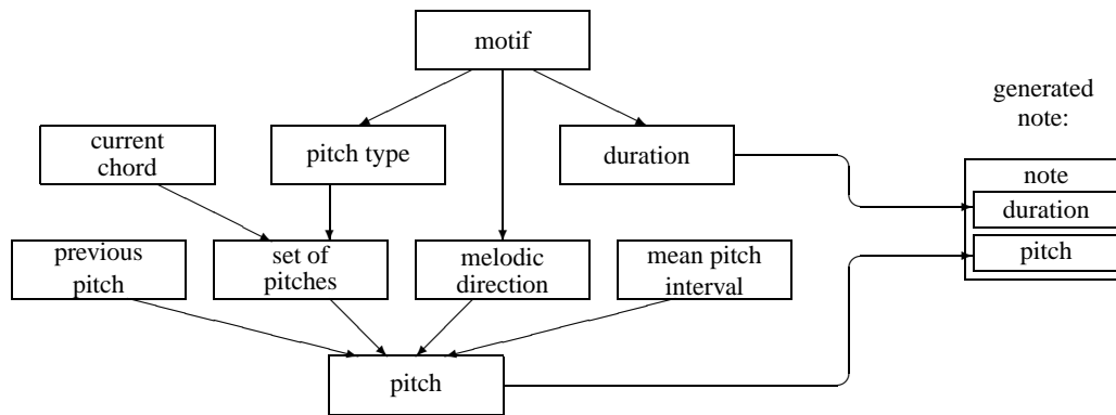
Figure 2: Block diagram of note generation during motif process
