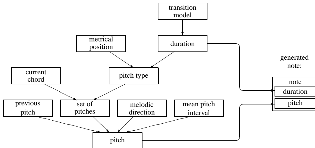
Figure 1: Block diagram of note generation during meloding process
