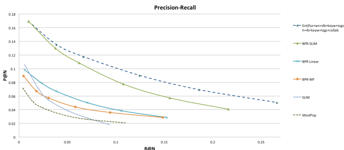
Figure 1: Precision-Recall results.
